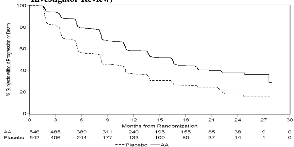
Figure 4: Kaplan Meier curves of radiographic progression-free survival in patients treated with either abiraterone acetate or placebo in combination with prednisone or prednisolone plus LHRH analogues or prior orchiectomy (At second interim analysis of OS-Investigator Review)
