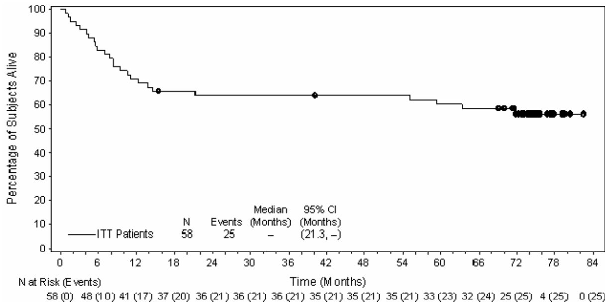
Figure 9: Kaplan-Meier Plot of OS
