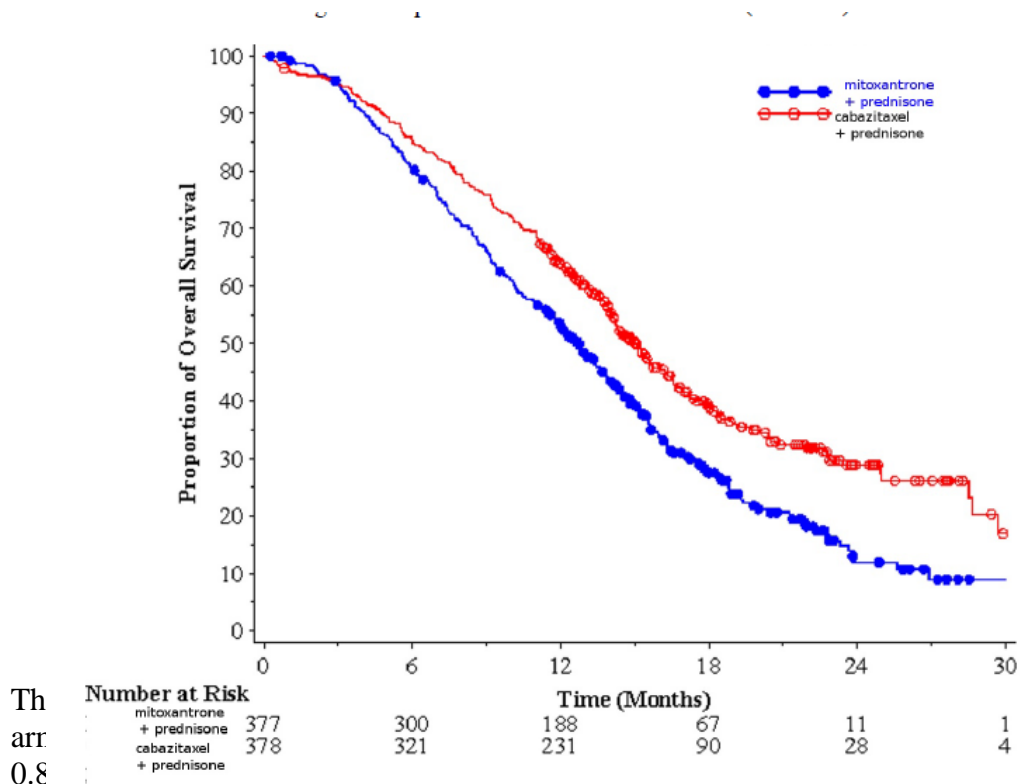
Figure 1: Kaplan Meier overall survival curves (EFC6193)
