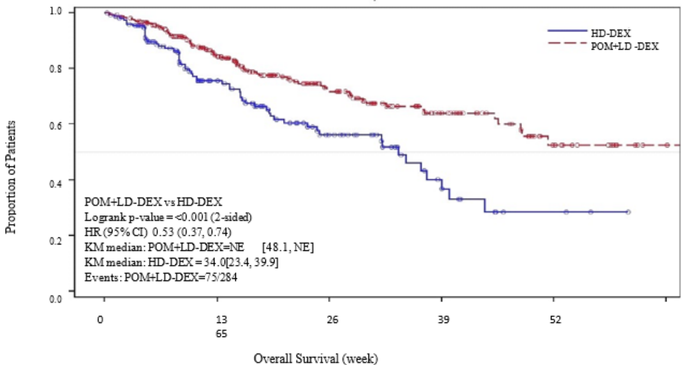
Figure 3. Kaplan-Meier Curve of overall survival (ITT Population)
