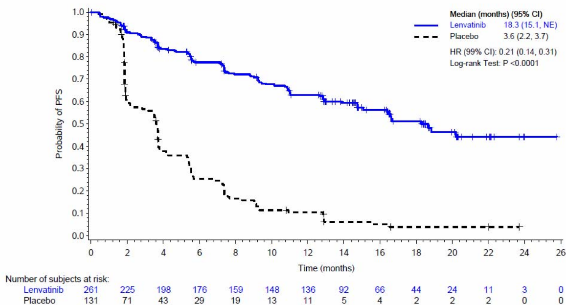
Figure 1 Kaplan-Meier Curve of Progression-Free Survival - DTC
