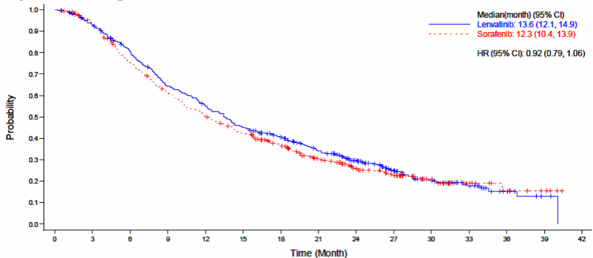
Figure 2 Kaplan-Meier Curve of Overall Survival - HCC
