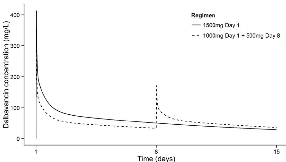
Figure 1: Dalbavancin Plasma Concentrations versus time in a typical adult ABSSI patient (simulation using population pharmacokinetic model) for both the single and the two-dose regimens
