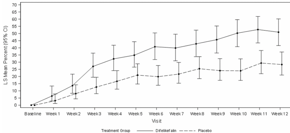
KALM-2
