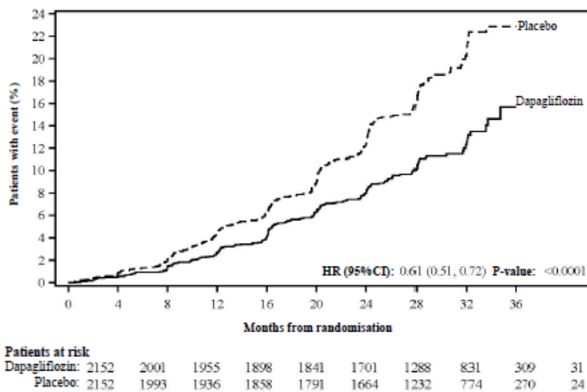
Figure 7: Time to first occurrence of the primary composite endpoint, \geq 50\% sustained decline in eGFR, end-stage kidney disease, cardiovascular or renal death
